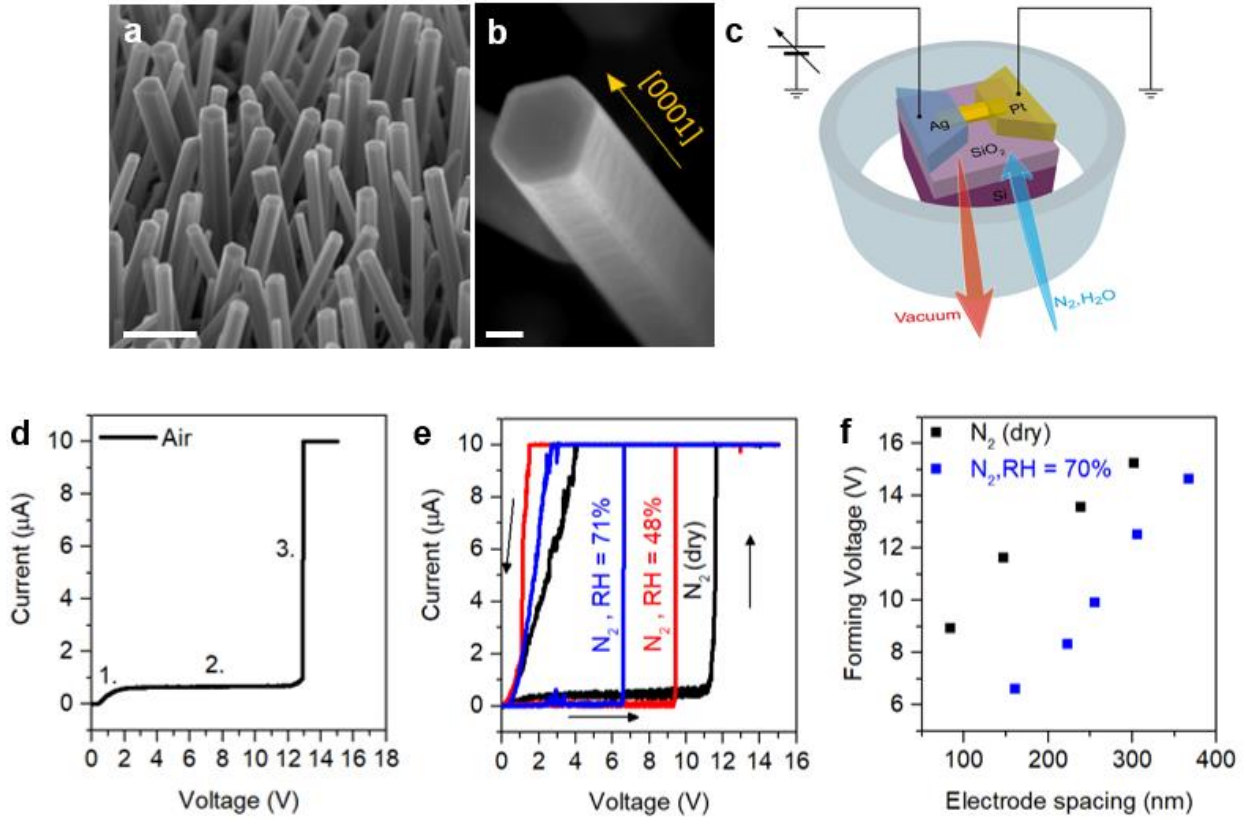
Figure. 1. ZnO NW based memristive device and influence of moisture on electroforming. (a) SEM image of NW arrays after the growth process (scale bar, 500 nm) and (b) detail of a single ZnO NW with hexagonal shape grown along the [0001] polar direction (scale bar, 40 nm) (c) Schematic representation of a single NW based memristive device with electrical connections in an atmosphere-controlled chamber. (d) Typical electroforming process of a single NW memristive cell in air, evidencing a diode-like behaviour for V < 1.5V (1.), current saturation regime for higher voltages (2.) and an abrupt change in resistance due to the formation of an Ag conductive path (3.). (e) Comparison of the electroforming curves of NW memristive cells with same electrode spacing (~ 150 nm) in N 2 environment at different levels of moisture showing a reduction of the forming
